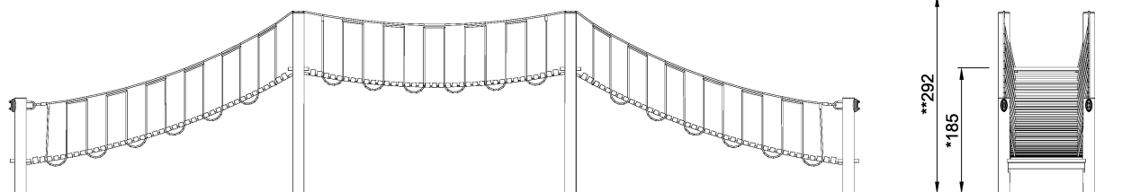
COR641201 1:100
