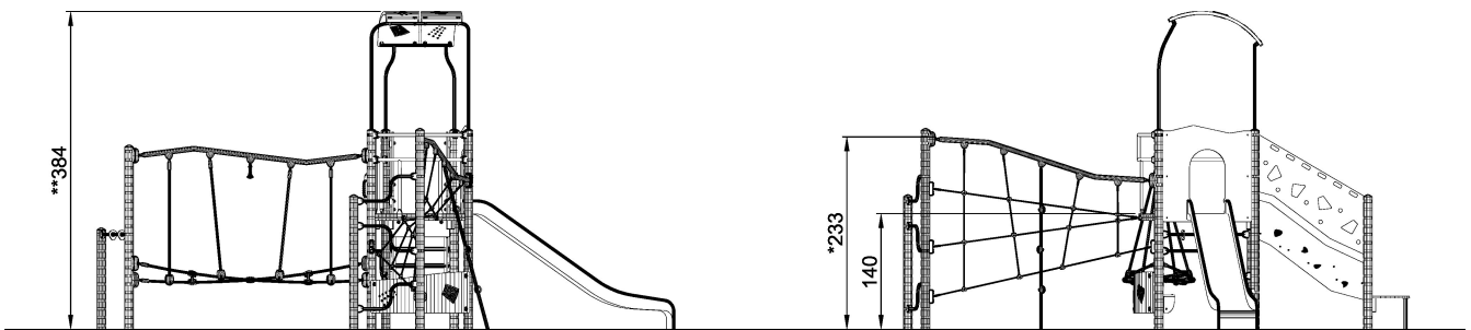
ELE500010 1:100
