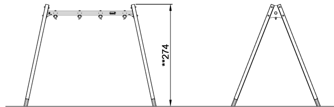
KSW902 1:100
